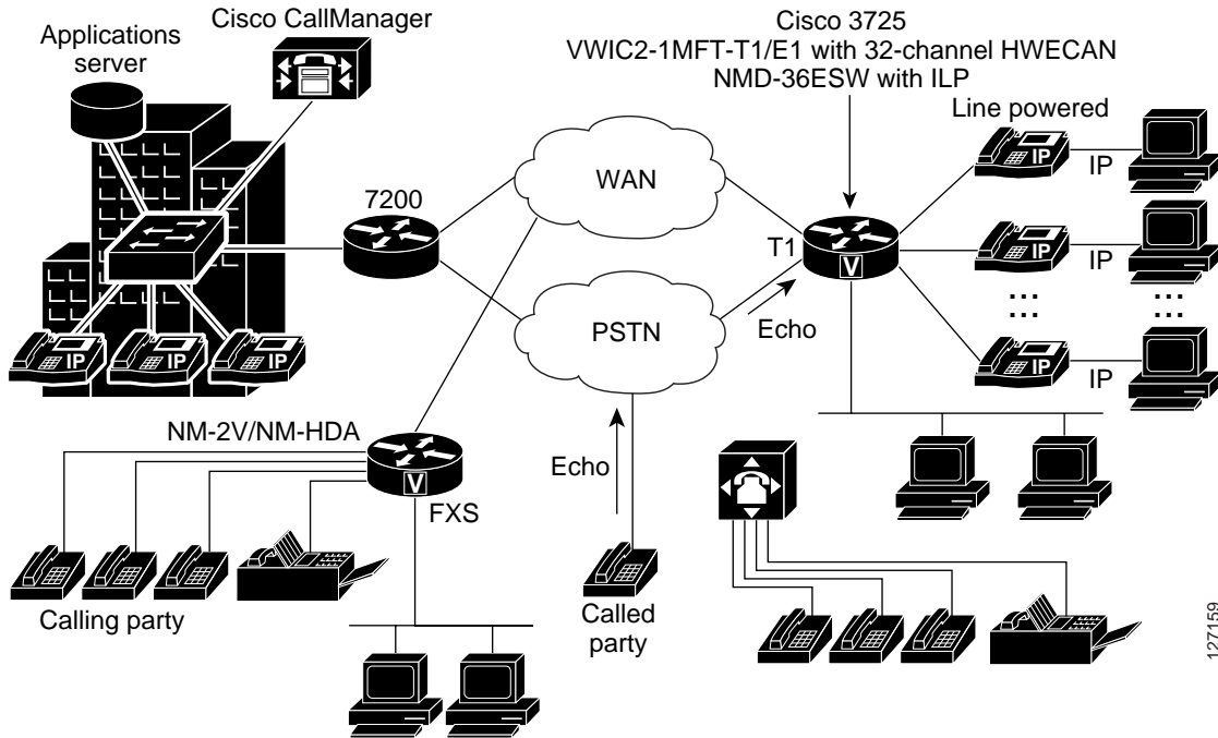
Figure 1 Sample Network Topology for the Second-Generation 1- and 2-Port T1/E1 Multiflex Trunk Voice/WAN Interface Cards
